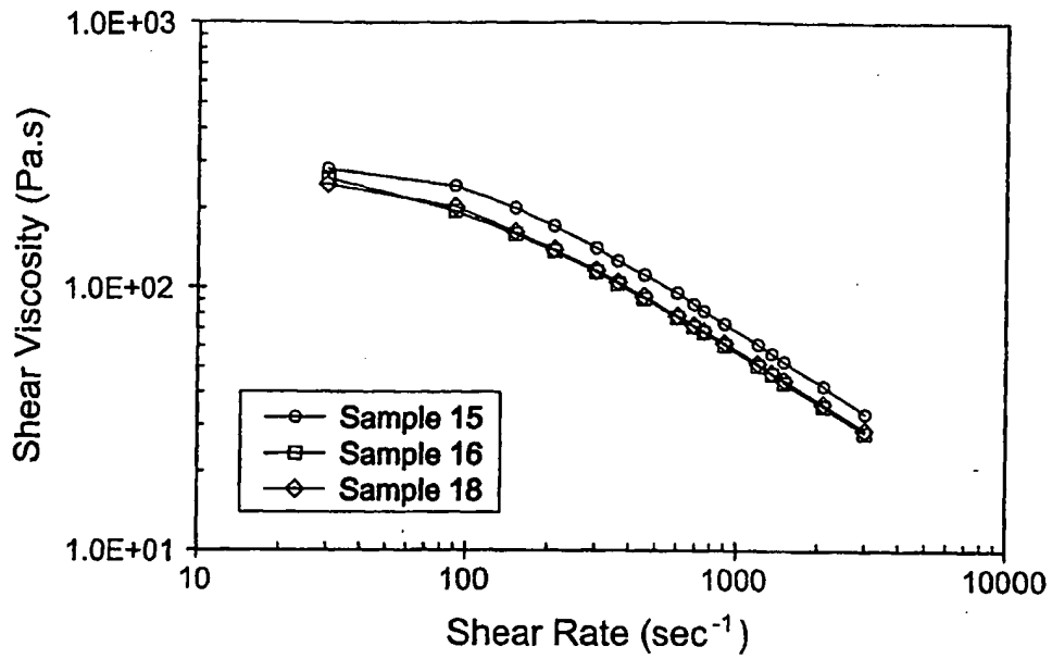
Fig. 13 Shear Viscosity of Plasticized Propylene Impact Copolymers
